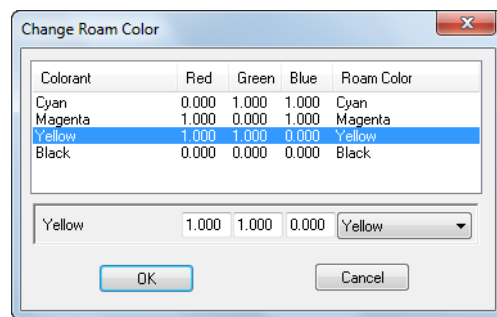
Figure 13.19 Change Roam Color dialog box
